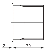
矩形外花键轴D 10-72d11x82d11x12f8
