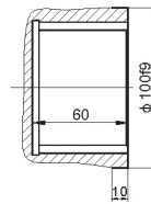
矩形内花键轴I 10-72D11x82D11x12H9
